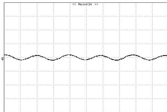
Figure 11: Input Terminal Ripple Current, i_c , at full rated output current and nominal input voltage with 12uH source impedance and 33uF electrolytic capacitor (200 mA/div, 1us/div)
