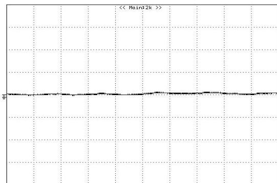
Figure 12: Input reflected ripple current, i_s , through a 12uH source inductor at nominal input voltage and rated load current (20 mA/div, 1us/div)
