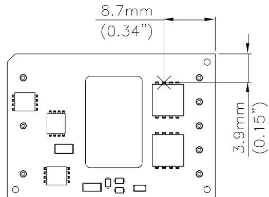
Figure 20: Temperature measurement location
