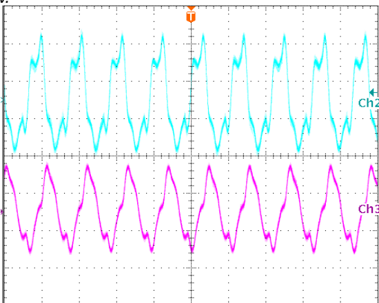
Output voltage ripple at nominal input voltage and max load current Top trace +15V, 10 mV/div, Bottom trace -15V, 10mV/div, 2us/div. Load cap: 10 \mu F, tantalum capacitor and 1 \mu F ceramic capacitor. Bandwidth: 20 MHz.
