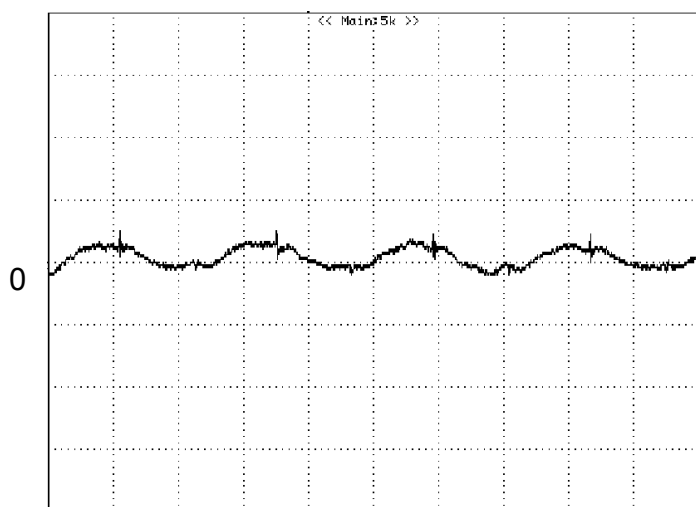
Figure 14: Output voltage ripple at nominal input voltage and rated load current ( I_o=10\text{A} ) (20 mV/div, 1 \mu\text{s} /div) Load capacitance: 1\mu\text{F} ceramic capacitor and 10\mu\text{F} tantalum capacitor. Bandwidth: 20 MHz. Scope measurements should be made using a BNC cable (length shorter than 20 inches). Position the load between 51 mm to 76 mm (2 inches to 3 inches) from the module
