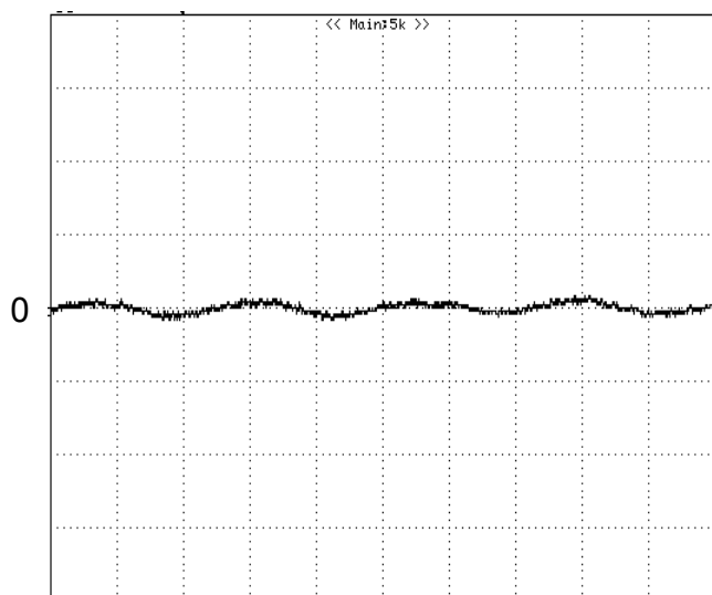
Figure 12: Input reflected ripple current, i_s , through a 12\mu\text{H} source inductor at nominal input voltage and rated load current (20 mA/div, 1 \mu\text{s} /div)
