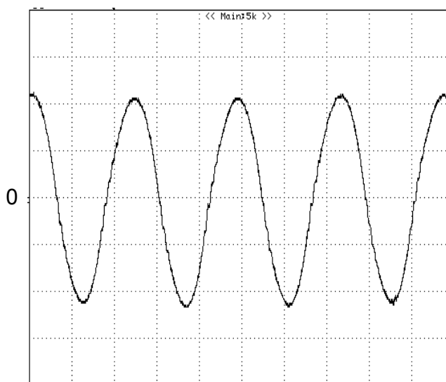
Figure 11: Input Terminal Ripple Current, i_c , at full rated output current and nominal input voltage with 12\mu H source impedance and 33\mu F electrolytic capacitor (50 mA/div, 1us/div)
