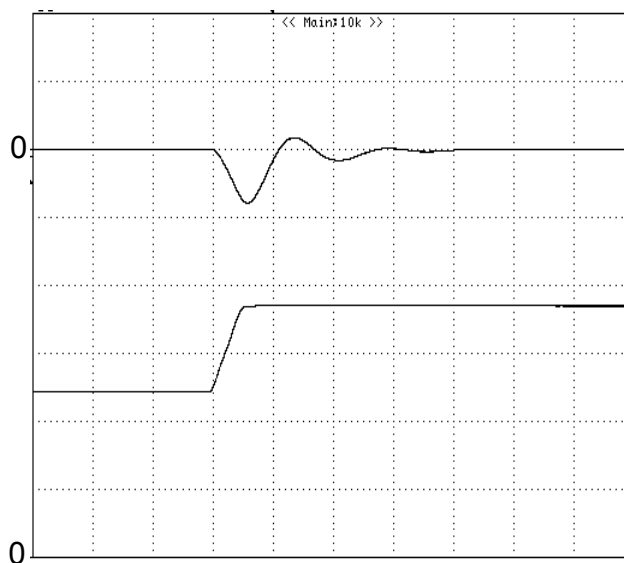
Figure 9: Output voltage response to step-change in load current (50%-75% of I_o , max; di/dt = 0.1A/\mu s ). Load cap: 10\mu F tantalum capacitor and 1\mu F ceramic capacitor. Top Trace: V_{out} (100mV/div, 50us/div), Bottom Trace: I_{out} (2A/div). Scope measurement should be made using a BNC cable (length shorter than 20 inches). Position the load between 51 mm to 76 mm (2 inches to 3 inches) from the module
