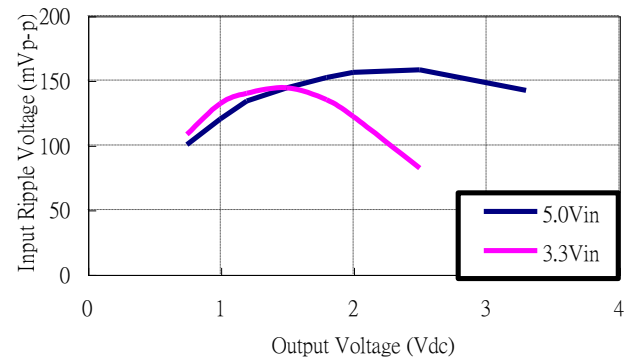
Figure 32: Input voltage ripple for various output models, I_O = 10 \text{ A} ( C_{IN} = 2 \times 100 \text{ µF} tantalum // 47 \text{ µF} ceramic)
