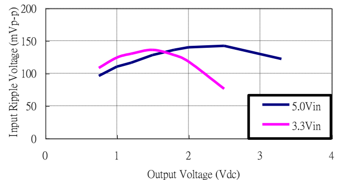
Figure 33: Input voltage ripple for various output models, I_O = 10 \text{ A} ( C_{IN} = 4 \times 100 \text{ µF} tantalum // 2 \times 47 \text{ µF} ceramic)
