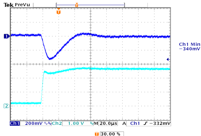
Figure 24: Typical transient response to step load change at 2.5A/\mu s from 50% to 100% of I_o , max at 3.3Vin, 2.5V out (Cout = ceramic, 10μF tantalum)
