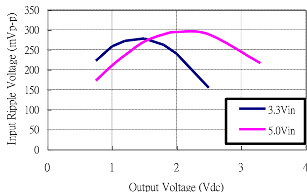
Figure 32: Input voltage ripple for various output models, I_O = 16 \text{ A} ( C_{IN} = 2 \times 100 \text{ } \mu\text{F} tantalum // 47 µF ceramic)
