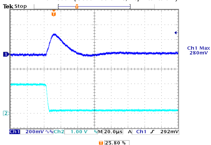
Figure 25: Typical transient response to step load change at 2.5A/\mu s from 100% to 50% of I_o , max at 3.3Vin, 1.8V out (Cout = ceramic, 10μF tantalum)
