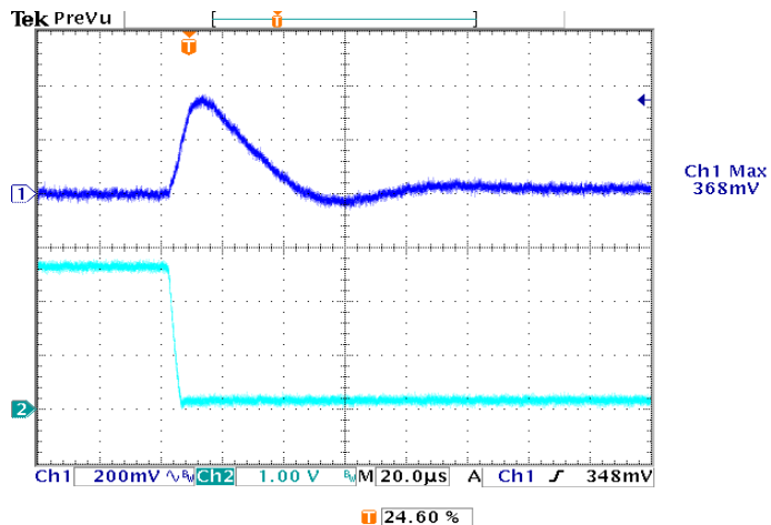
Figure 23: Typical transient response to step load change at 2.5A/\mu s from 100% to 50% of I_o , max at 3.3Vin, 2.5V out (Cout = ceramic, 10μF tantalum)
