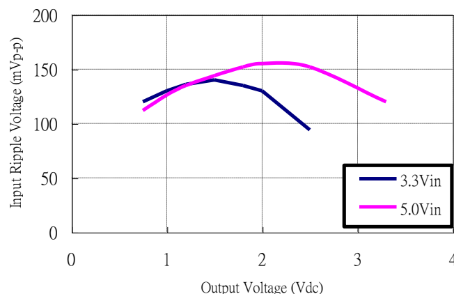
Figure 33: Input voltage ripple for various output models, I_O = 16 \text{ A} ( C_{IN} = 4 \times 100 \text{ } \mu\text{F} tantalum // 2 x 47 µF ceramic)
