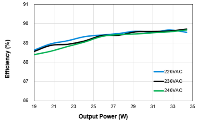
LNP-08A35WBCA – 800mA
