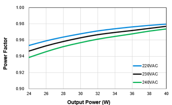
LNP-10A35WBCA/B – 1050mA
