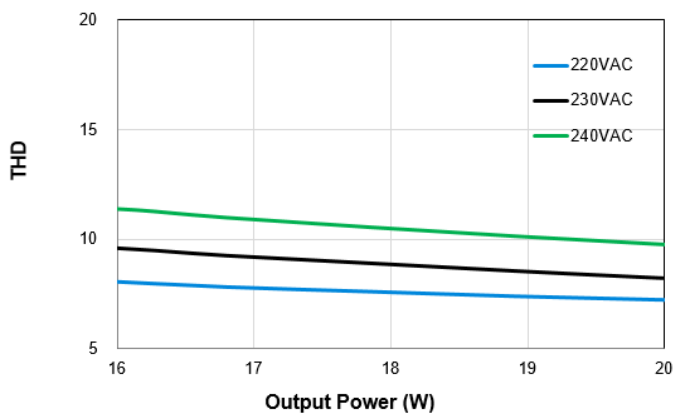
LNP-05A20WBCA – 500mA
