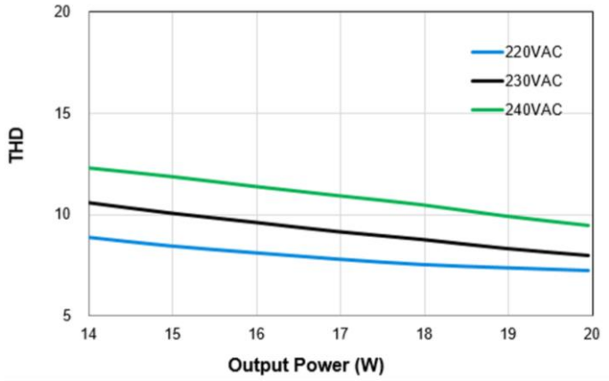
LNP-03A21WBCA – 350mA
