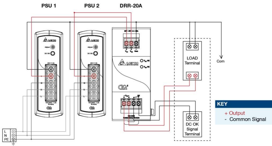
Fig. 2 Redundancy / Parallel Operation Connection Diagram
