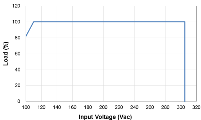
OUTPUT LOAD VS INPUT VOLTAGE
