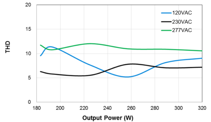
USCO-320210GA – 2100mA
