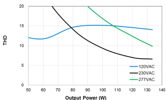
USCO-200140GA – 700mA
