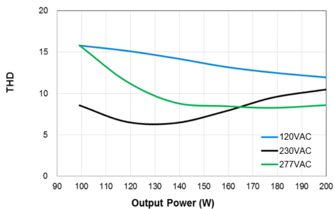
USCO-200140GA – 1400mA
