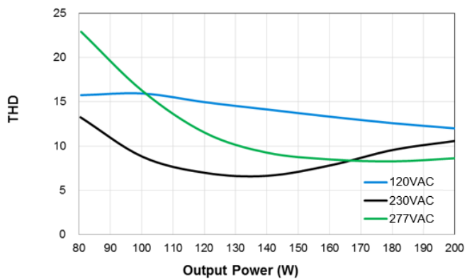
USCO-200140GA – 1050mA
