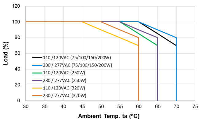
OUTPUT LOAD VS AMBIENT TEMPERATURE
