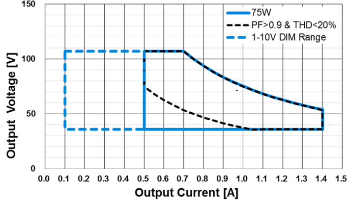
Output Voltage Range - 75W
