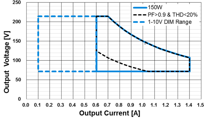
Output Voltage Range - 150W
