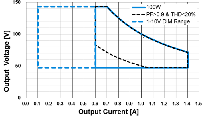
Output Voltage Range - 100W
