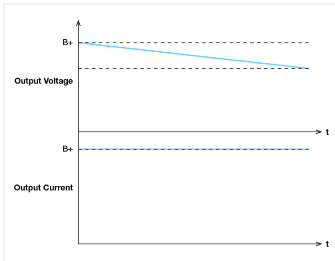
Buffering Mode (Battery discharging (B+))
