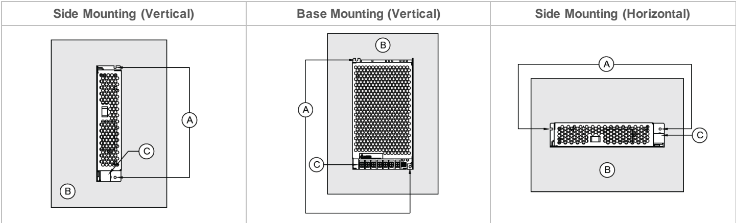
Fig. 4 Mounting Orientation
