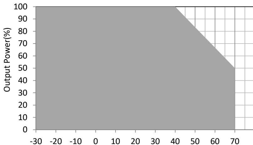
Fig. 1 De-rating for Vertical and Horizontal Mounting Orientation > 40^{\circ}\text{C} de-rate power by 1.67\% / ^{\circ}\text{C}
