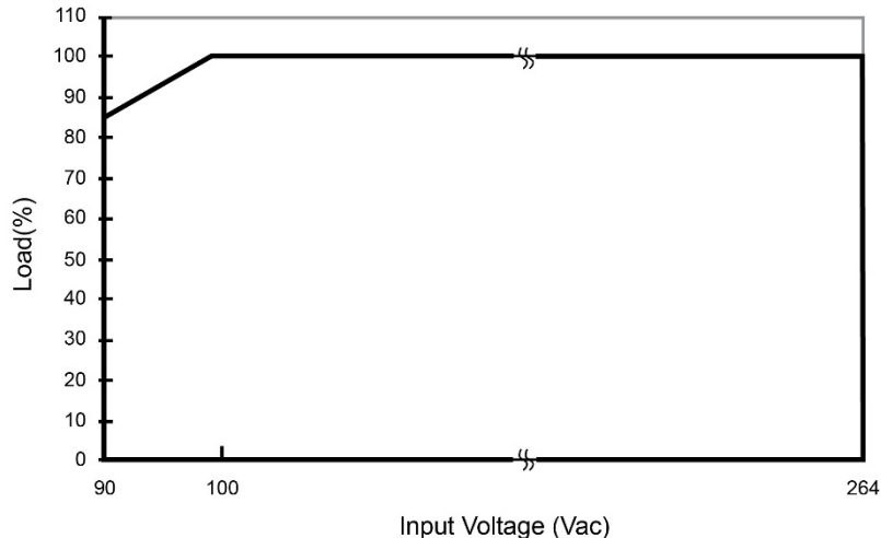
Fig. 2 De-rating for AC Input Voltage < 100\text{ Vac} de-rate power by 1.33\% / \text{V}
