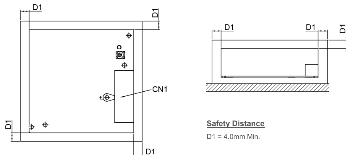
Fig. 3 Assembly Reference
