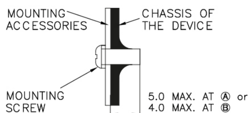
Fig. 4 Assembly Reference
