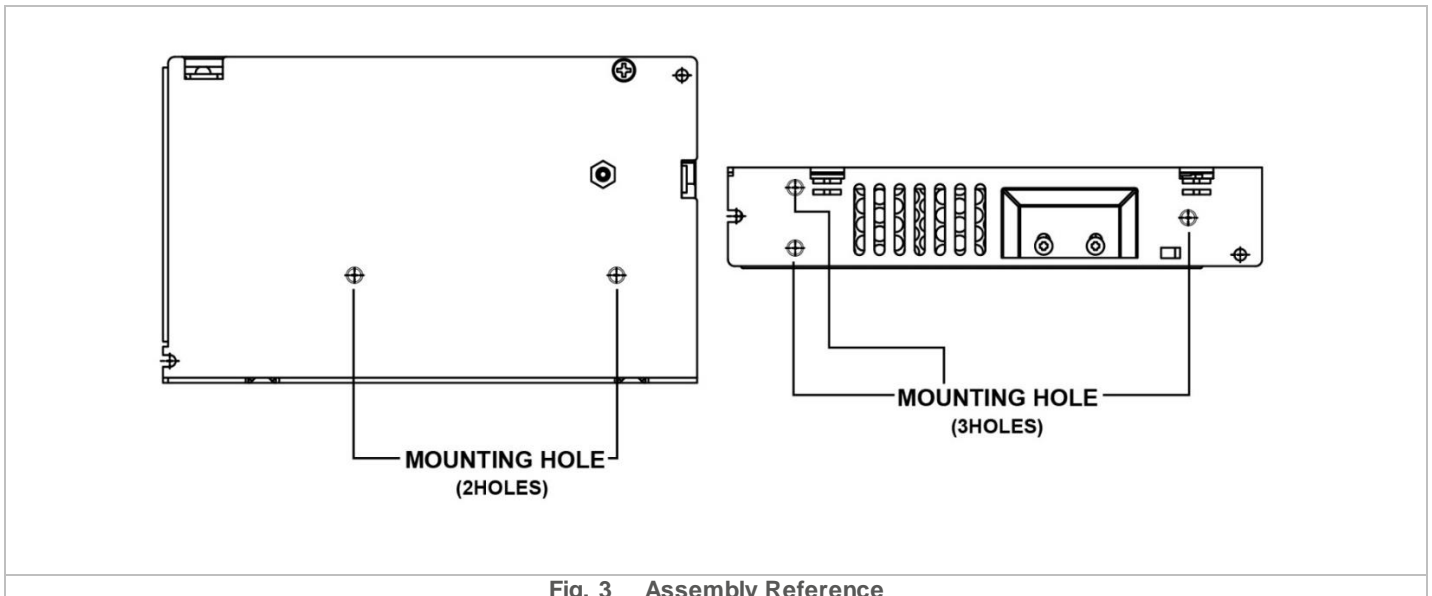
Fig. 3 Assembly Reference
