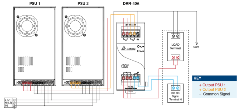
Fig. 5 Redundant Operation Connection Diagram
