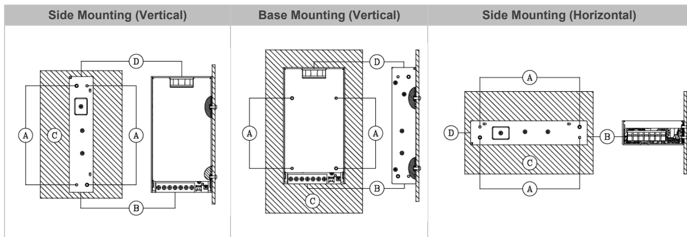
Fig. 2 Mounting Orientation
