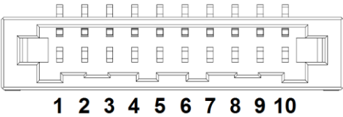
Fig. 4 Pin Assignment of CN101
