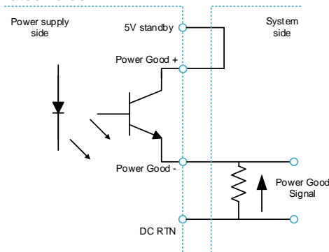
Figure 8. Power Good Connection
