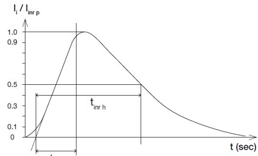
Figure 6. Inrush Current
