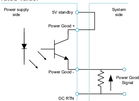
Figure 8. Power Good Connection
