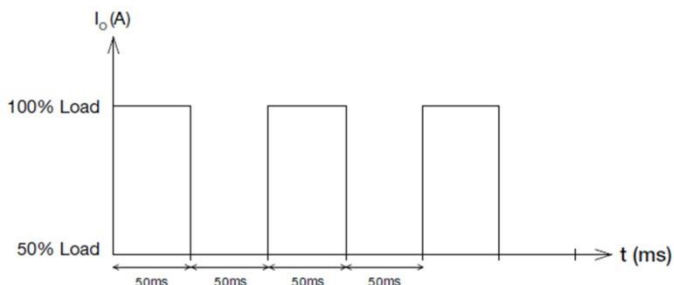
Figure 5. Dynamic Load
