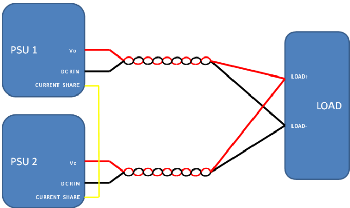
Fig. 10: Parallel connection
