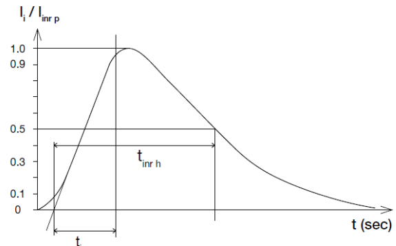
Figure 7. Inrush Current
