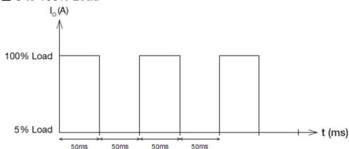
Figure 6. Dynamic Load
