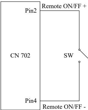
Figure 9. Remote On/Off Connection
