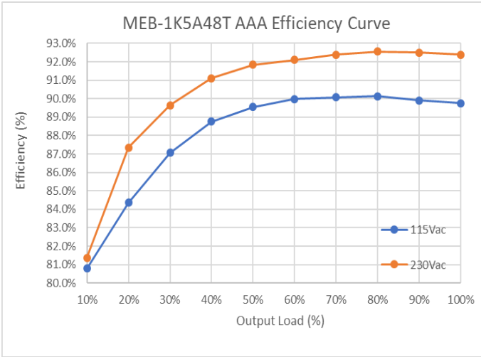
Figure 1-2. Typical efficiency Curve for MEB-1K5A48T AAA
