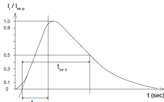
Figure 7. Inrush Current
