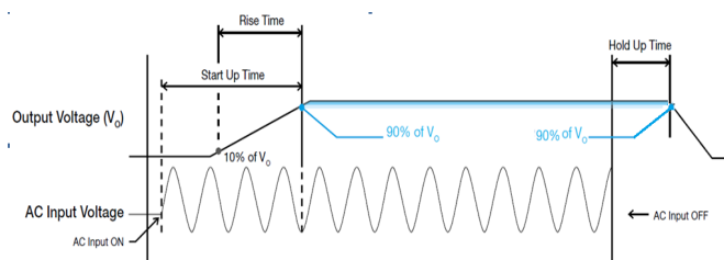
Figure 5. Time sequence
