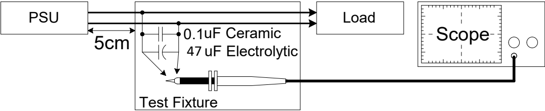
Figure 2. Ripple & Noise testing set up
