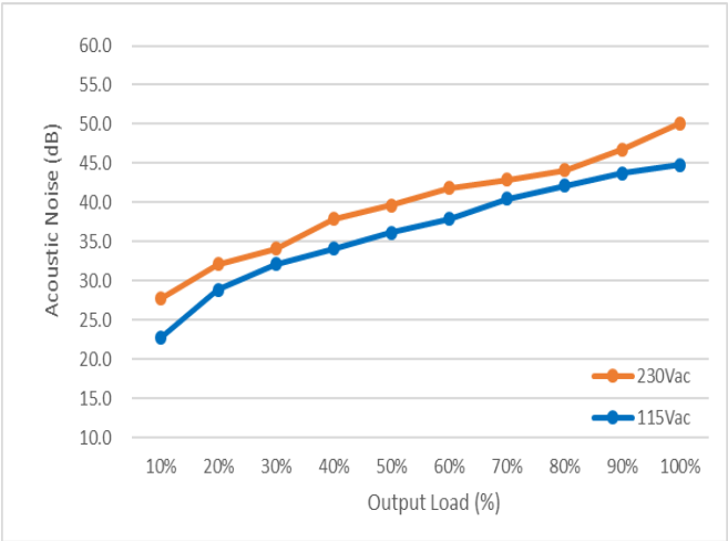
Figure 3-3. Typical acoustic noise curve for MEB-1K5A48T AAA
