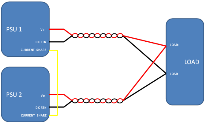
Fig. 10: Parallel connection
