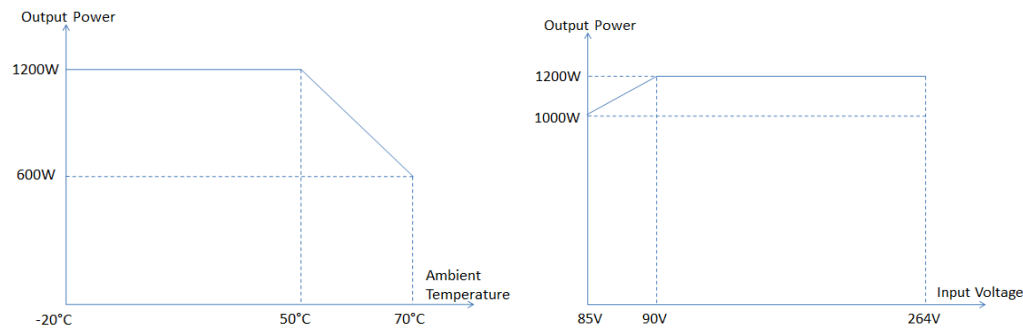
Power De-rating curve
