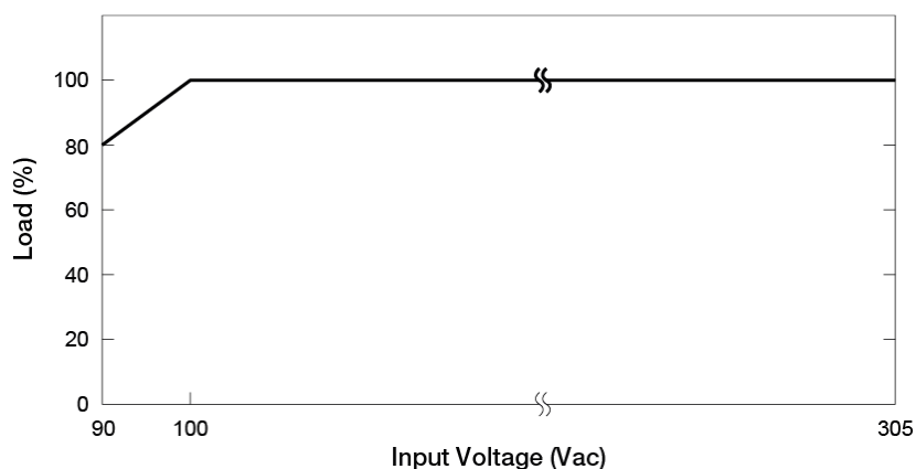
Fig. 2 De-rating for Low Input Voltage (All Models) < 100\text{Vac} de-rate power by 2% / Vac
