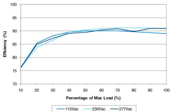
LNE-36V150W□
