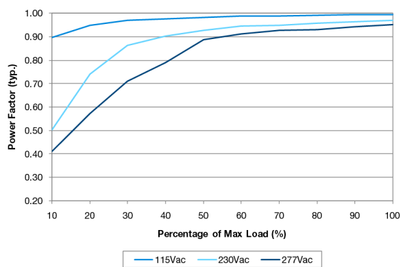
LNE-36V150W□
