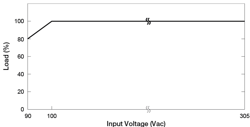
Fig. 2 De-rating for Low Input Voltage (All Models) < 100\text{Vac} de-rate power by 2\% / \text{Vac}
