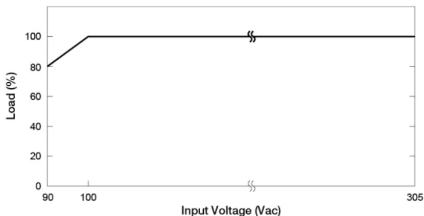
Fig. 2 De-rating for Low Input Voltage (All Models)
