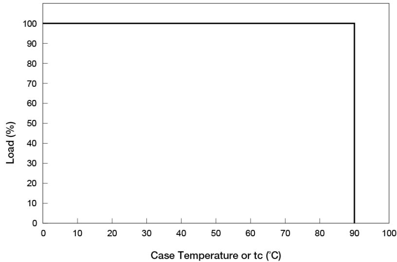
Output Load VS LED Driver Case Temperature
