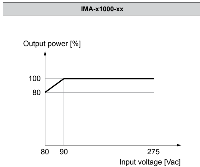
Fig. 7: Output power versus input voltage
