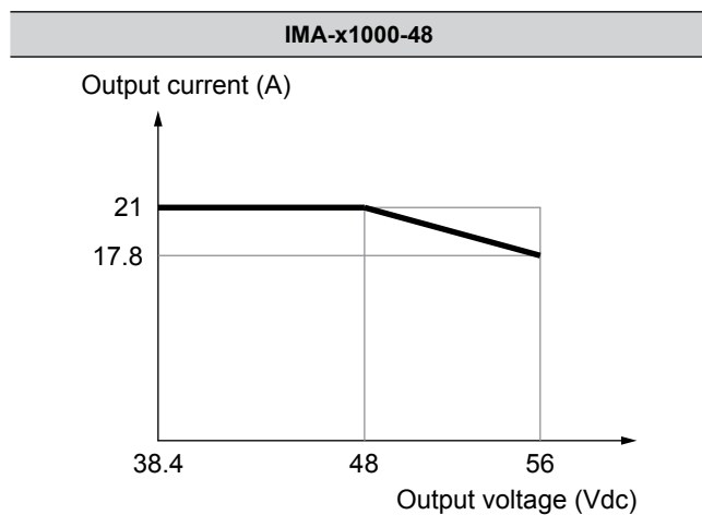
Fig. 11: Output current versus output voltage 48 V
