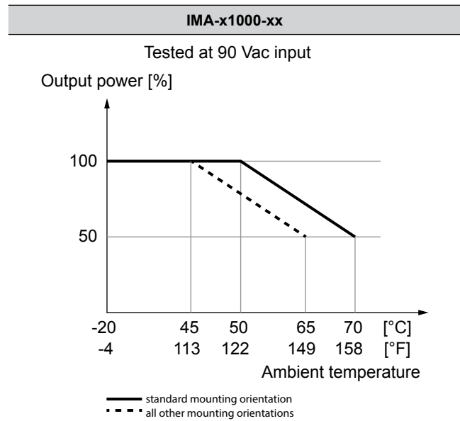
Fig. 8: Output power versus ambient temperature
