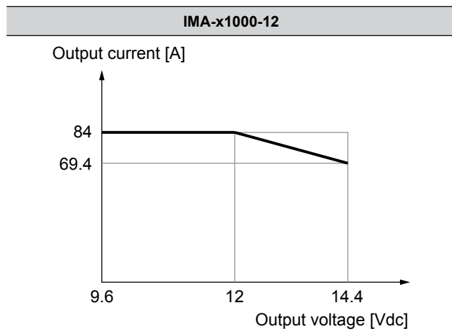
Fig. 9: Output current versus output voltage 12 V
