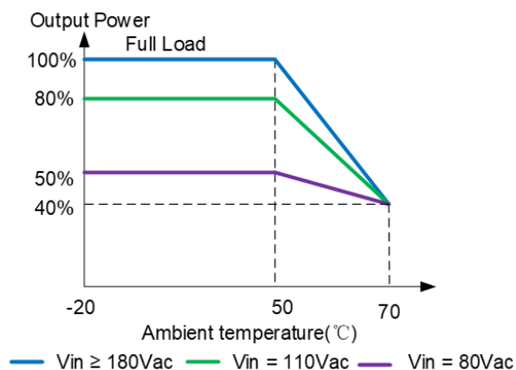
Fig. 8: Output power versus ambient temperature
