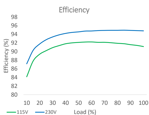
Fig. 12: Typical efficiency curves 48 V
