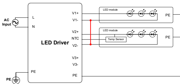
Misconnection of all 2 output negative terminals together.
