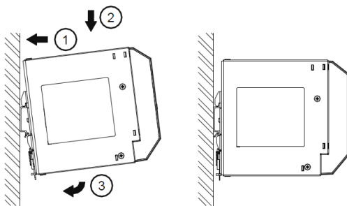
Fig. 6.1 Mounting
