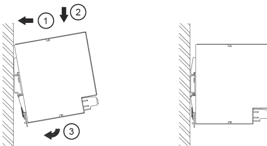
Fig. 3.1 Mounting
