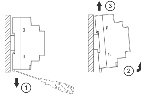
Fig. 3.2 Dismounting
