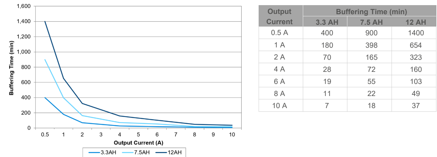
Fig. 1 Buffering Time VS. Output Current
