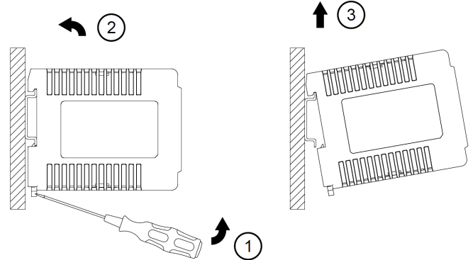
Fig. 2.2 Dismounting
