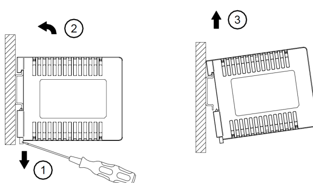
Fig. 2.2 Dismounting
