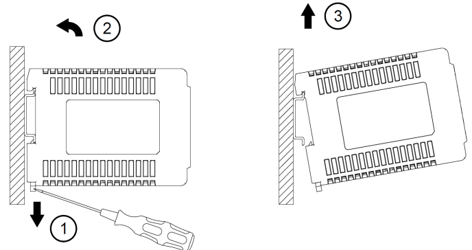
Fig. 2.2 Dismounting
