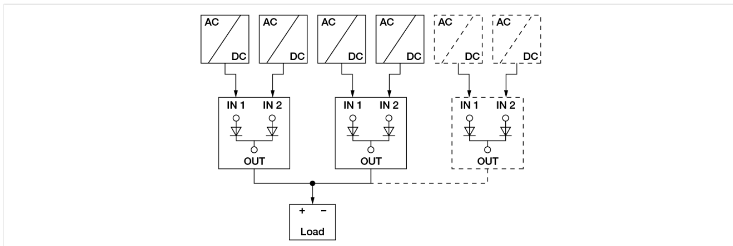
Fig. 3.3 N+1 Redundancy
