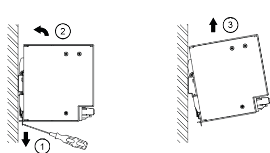
Fig. 2.2 Dismounting
