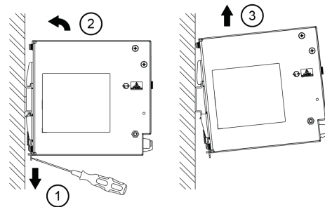
Fig. 6.2 Dismounting
