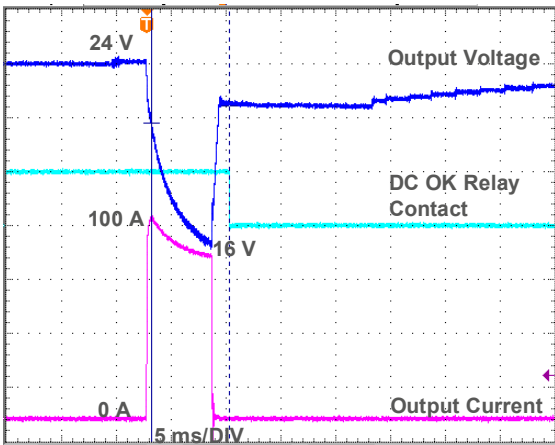
Fig. 8.3 APB 500% of nominal output current for 5 ms
