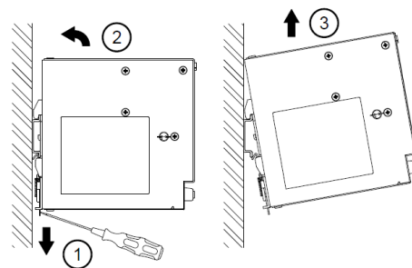
Fig. 6.2 Dismounting
