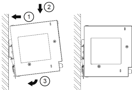
Fig. 6.1 Mounting
