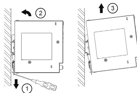
Fig. 6.2 Dismounting
