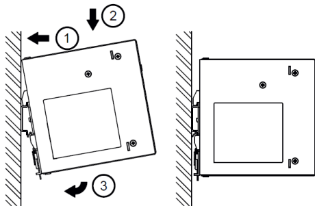
Fig. 3.1 Mounting
