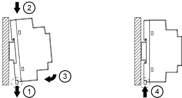
Fig. 2.1 Mounting
