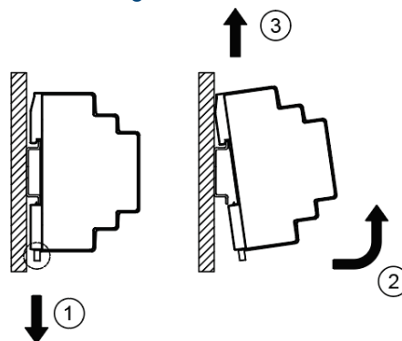
Fig. 2.2 Dismounting
