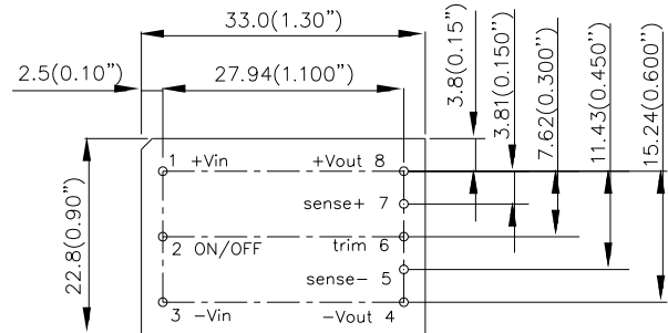
Through-hole module
