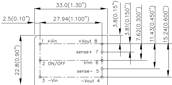
Surface-mount module
