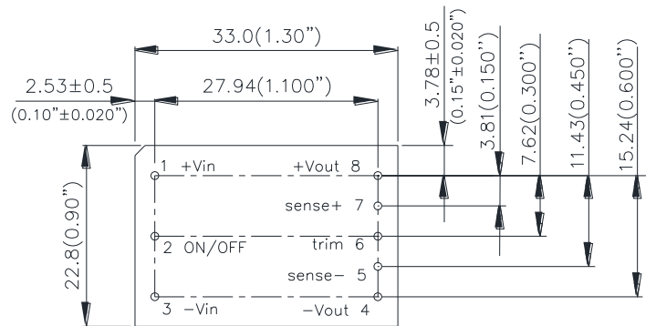
Through-hole module
