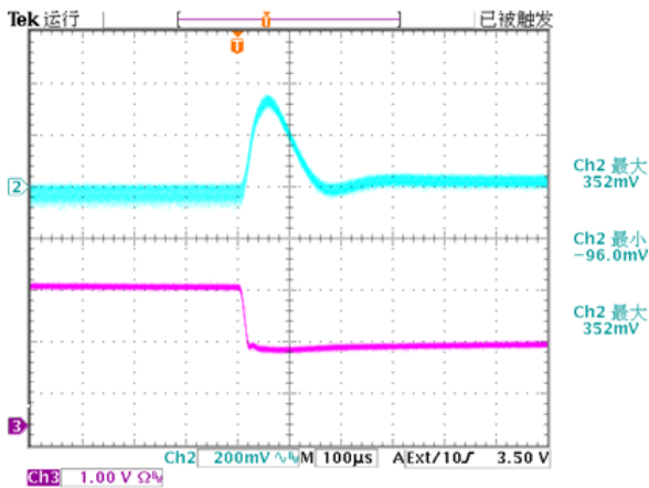
Figure 6: Output voltage response to step-change in load current (25%-50% of I_o , max; di/dt = 0.1A/\mu s ; V_{in} is 48v). Load cap: 10 \mu F tantalum capacitor and 1 \mu F ceramic capacitor. Top Trace: V_{out} (200mV/div, 100us/div), Bottom Trace: I_{out} (1A/div). Scope measurement should be made using a BNC cable (length shorter than 20 inches). Position the load between 51 mm to 76 mm (2 inches to 3 inches) from the module
