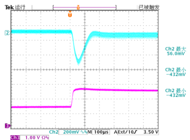
Figure 7: Output voltage response to step-change in load current (50%-25% of I_o , max; di/dt = 0.1A/\mu s ; V_{in} is 48v). Load cap: 10 \mu F tantalum capacitor and 1 \mu F ceramic capacitor. Top Trace: V_{out} (200mV/div, 100us/div), Bottom Trace: I_{out} (1A/div). Scope measurement should be made using a BNC cable (length shorter than 20 inches). Position the load between 51 mm to 76 mm (2 inches to 3 inches) from the module
