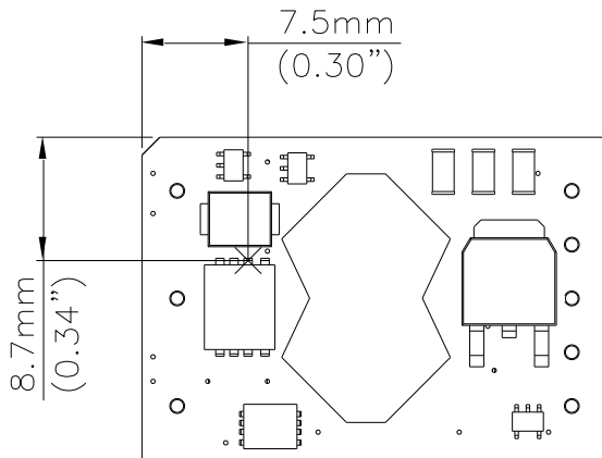
Figure 19: Hot spot1 temperature measurement location
