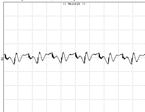
Figure 12: Output voltage ripple at nominal input voltage ( v_{in}=48v ) and rated load current ( I_o=10A ) (50 mV/div, 1 \mu s/div). Load capacitance: 1 \mu F ceramic capacitor and 100 \mu F tantalum capacitor. Bandwidth: 20 MHz. Scope measurements should be made using a BNC cable (length shorter than 20 inches). Position the load between 51 mm to 76 mm (2 inches to 3 inches) from the module
